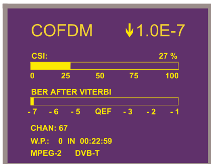
Figure 13.- BER measuring screen for COFDM-modulated signals Two measures are shown :
