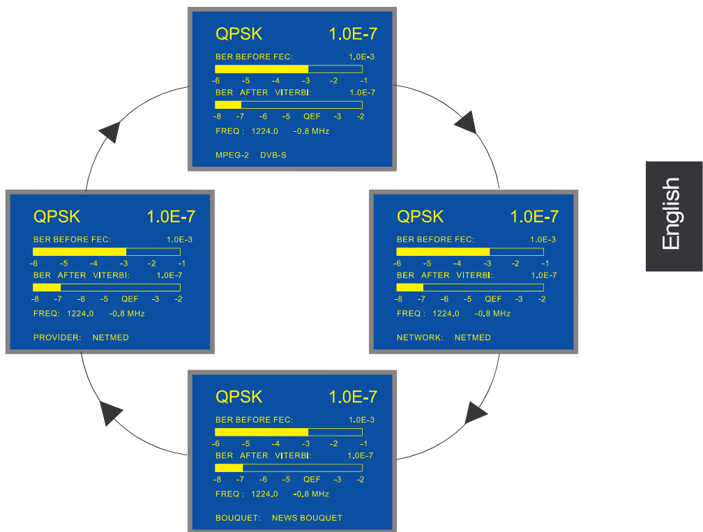
Figure 21.- DCI function. In this example the information coded by the operator on the Provider and Network fields is the same.
