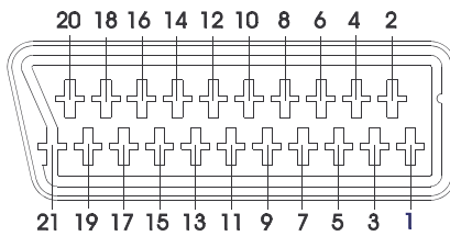
Figure 52.- Scart socket (external view).
