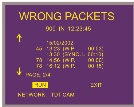
Figure 20.- W.P. measurement.
