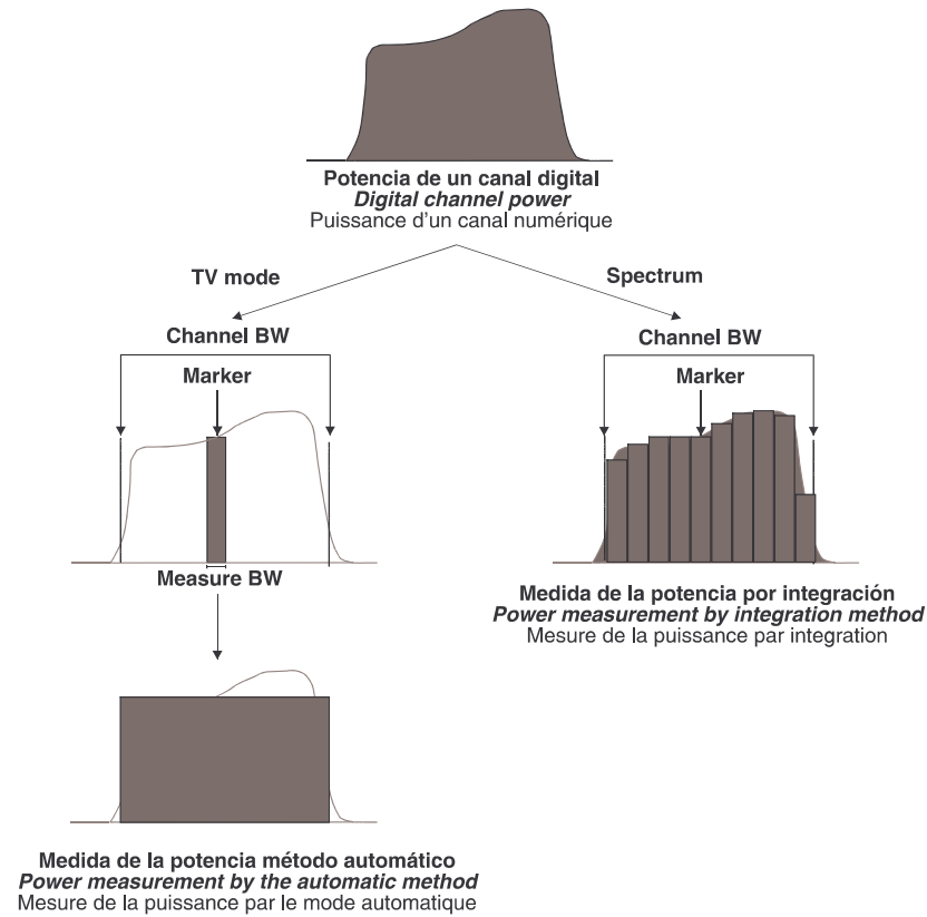
Figure 9.- Measuring digital power.
