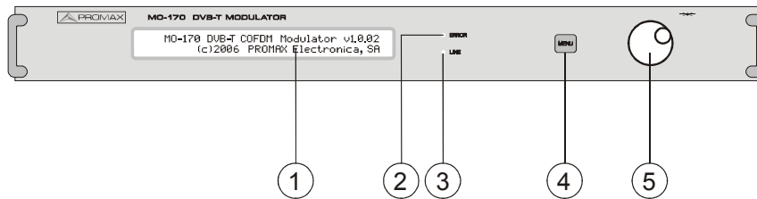
Figure 1.- Front panel.
